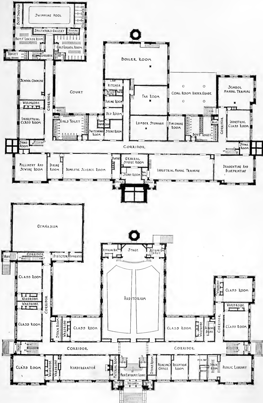
BASEMENT AND FIRST FLOOR PLANS DELAWARE SCHOOL, SYRACUSE, NEW YORK JAMES A. RANDALL, ARCHITECT
